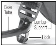
Figure 3 Hook Attachment
