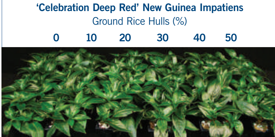
Fig. 2. Cuttings of ‘Celebration Deep Red’ New Guinea impatiens propagated in substrates containing 50 percent perlite and (from L to R) 0 to 50 percent ground rice hulls and 50 to 0 percent peat moss.
