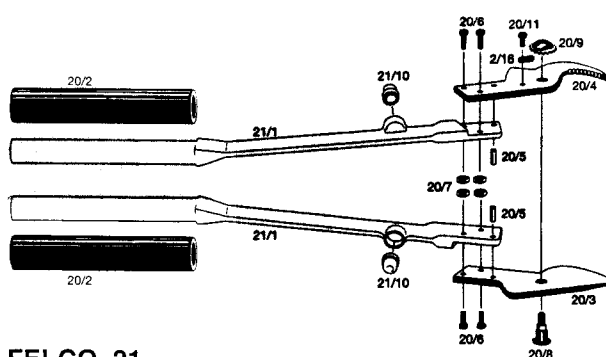
FELCO 21
